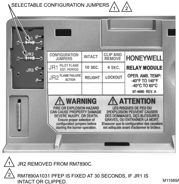
Fig. 4. Selectable site-configurable jumpers.
